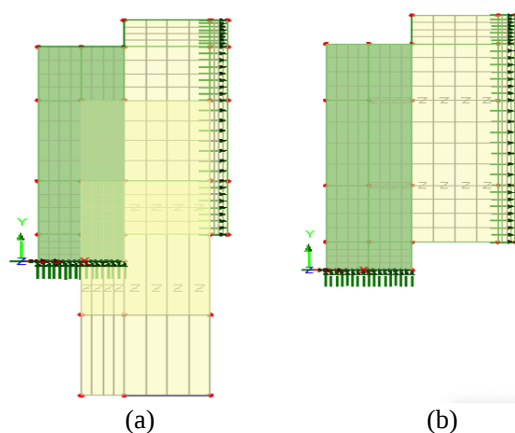
Figure V.- Process to assign the interface element between screw to timber/concrete. (a) Master (on timber/concrete) and slave (on screw) assignment and (b) Completed assignment of interface element
